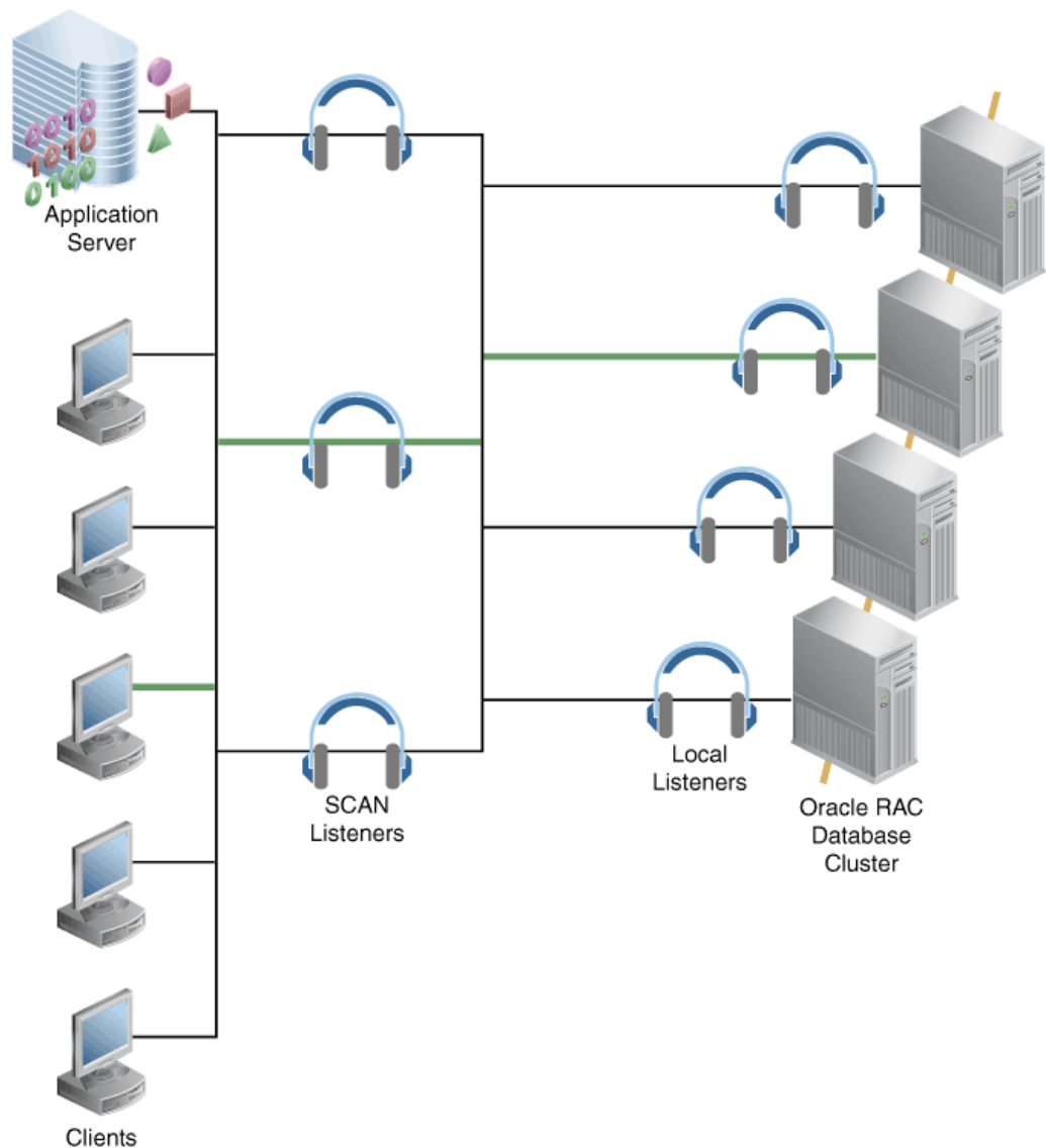
Figure 32-1 Connection Load Balancing Using the SCAN
